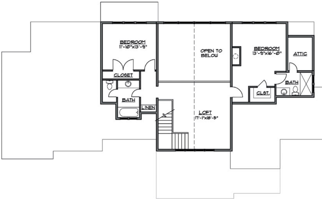
UPPER LEVEL 946 SQ. FT.
