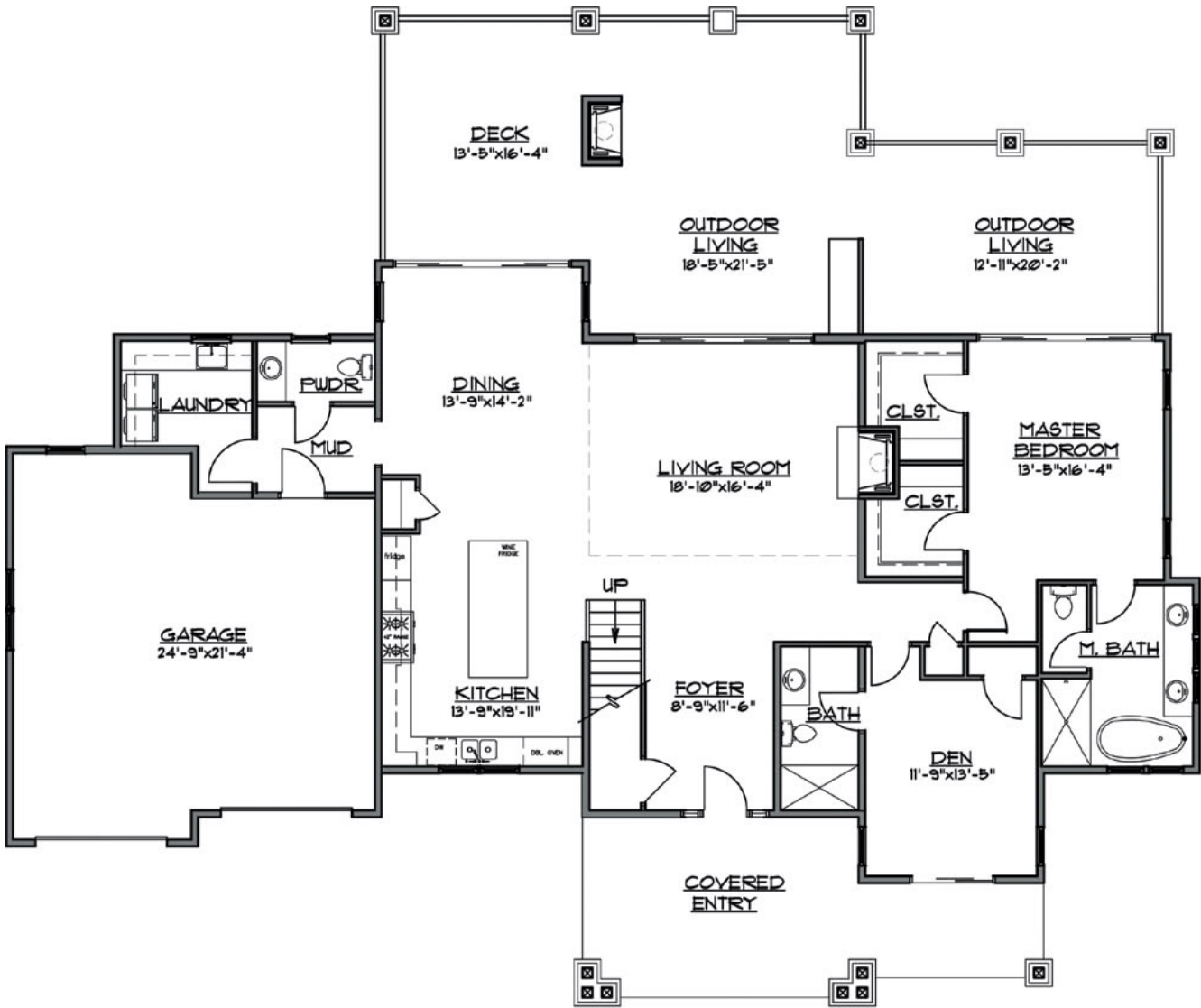
MAIN FLOOR 1,963 SQ. FT.
