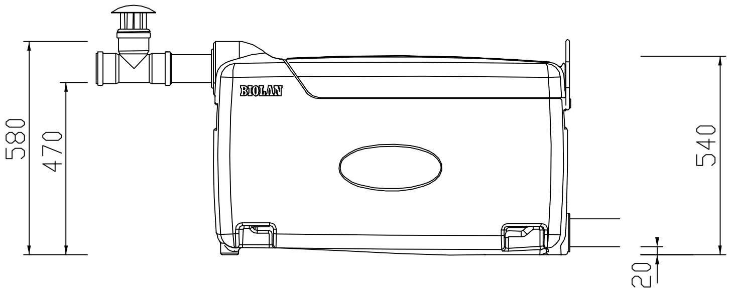
↑ Side view ↑
