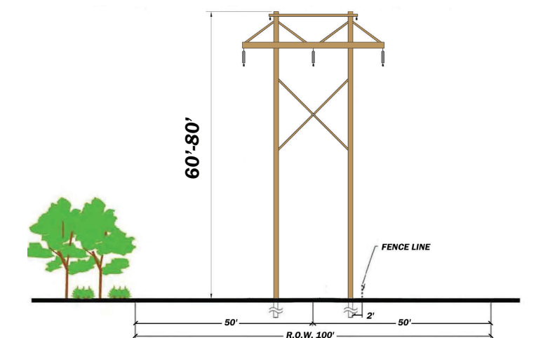
Typical 115kV Single Circuit, H-Frame Structure
