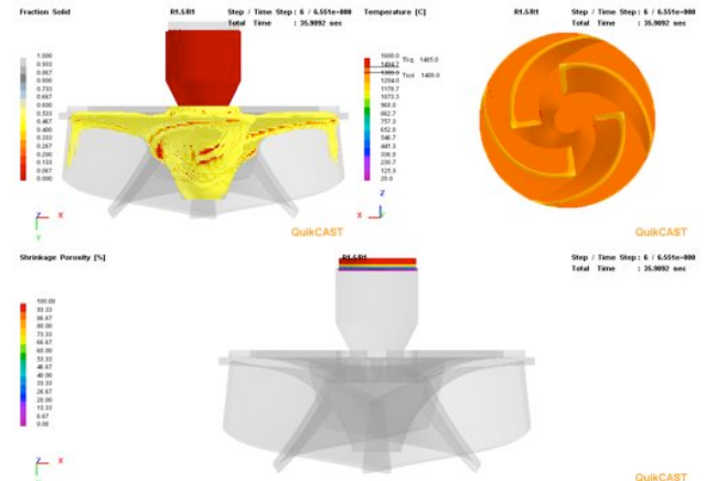
Foundry Melt Simulation
