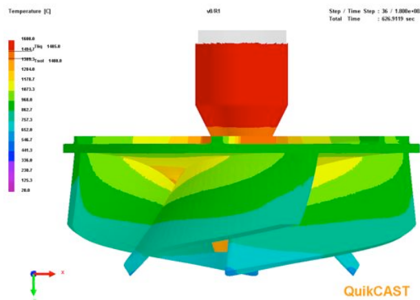
Foundry Cooling Simulation
