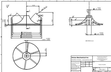
Machining Drawing
