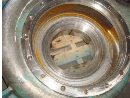
Worn Volute
