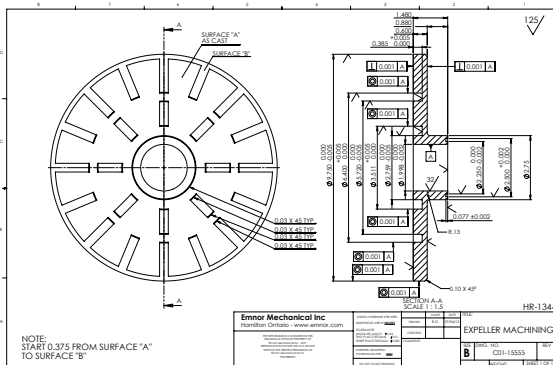
Machining Drawing
