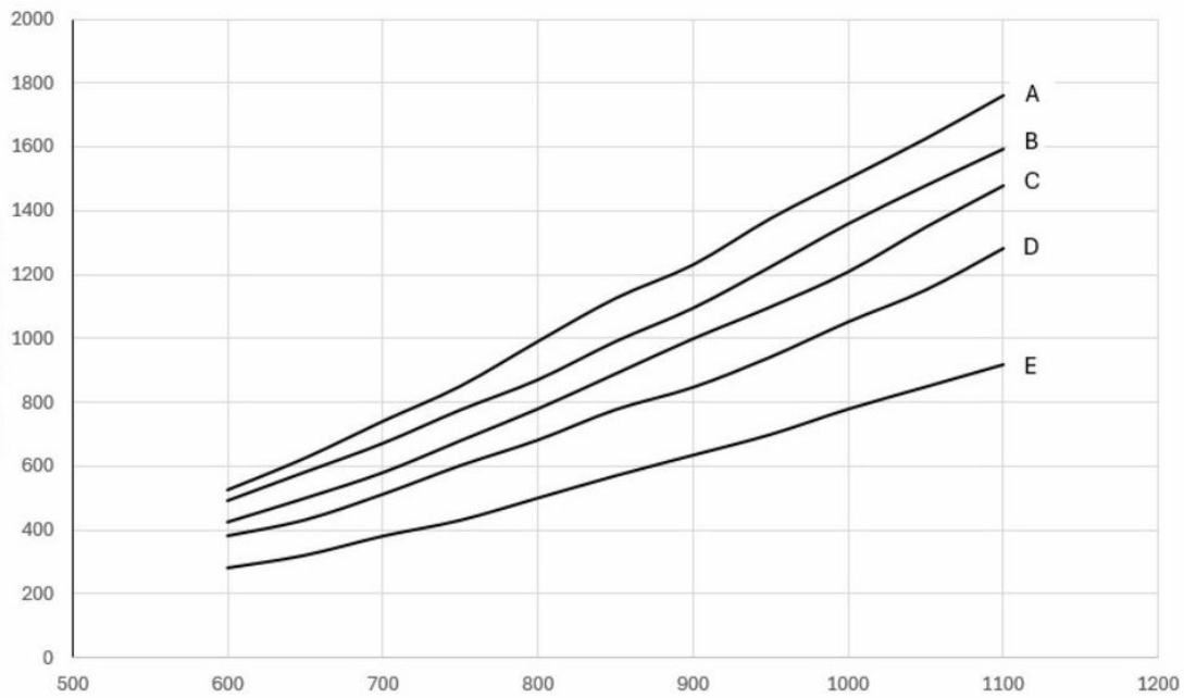
X: Airflow m 3 /h, Y: Static pressure Pa. A=5m Body work arm. B=4m Horizontal arm. C=4m Vertical arm. D=3m arm. E=2m arm
