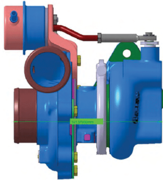
OVERALL LENGTH = 162.0 mm
