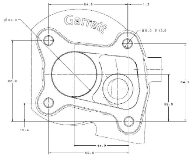
TURBINE OUTLET
