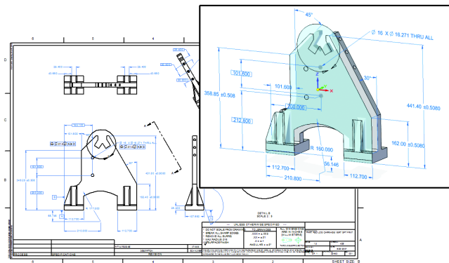
Figure 6. Designers can re-use 2D drawings and 3D parts more effectively with Solid Edge. Manufacturing dimensions of an imported 2D drawing can be automatically applied to its associated 3D model. The results allow designers to edit key parameters, such as distance between holes and overall dimensions.
