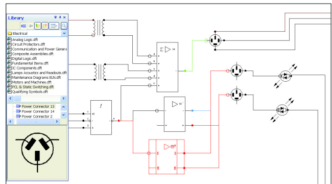
Figure 15. Schematic drawings can be easily created in Solid Edge. Deliverables include symbols for electrical, mechanical and piping that can be tied together with connectors. The above drawing indicates how elements update as blocks are moved.
