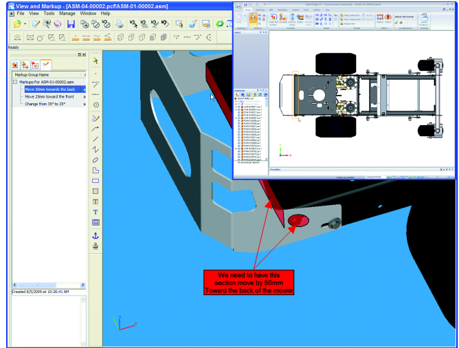
Figure 18. Design changes can be authored in a view and markup application. XpresReview, a free download, lets other users view and redline suggestions. Back in Solid Edge, the modification can be implemented with a simple fence stretch (inset).
