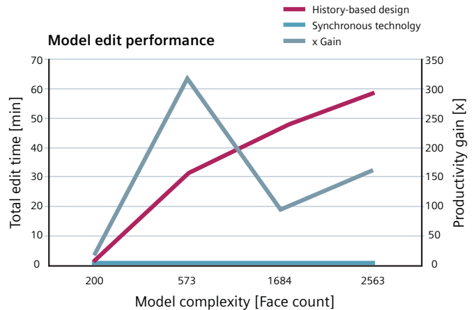
Figure 4. This chart compares performance between edits made in synchronous technology and a typical history-based modeling system. The difference is that synchronous technology edits the minimum amount of geometry, while edits in history-based systems often rebuild the entire model.
