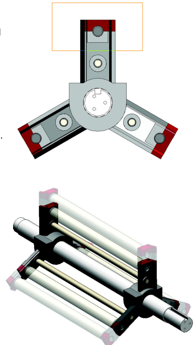
Figure 7. Designers can re-use assembly layouts and models more effectively with Solid Edge. Assembly edits across imported and native parts are done with a simple selected fence and drag. This is a familiar process for designers migrating from a 2D system. (Food mixing assembly courtesy of AMF Canada)
