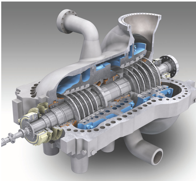
Figure 8. This HIP turbine assembly was modeled in Solid Edge and rendered with its advanced photorealistic rendering application. Material and lighting libraries let designers create life-like product images for customer presentations or promotional activities. (Image courtesy of POMIT Co., LTD, Korea)
