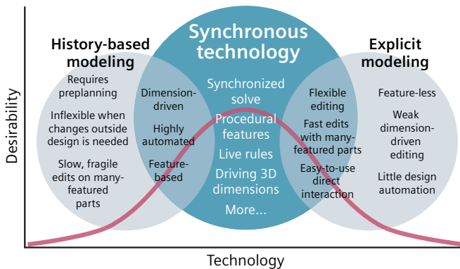
Figure 1. Synchronous technology and how it combines parametric design with explicit modeling for faster construction and change.
