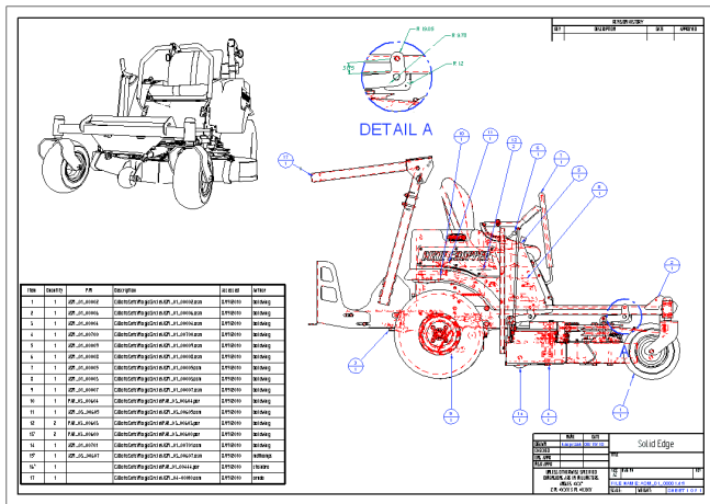
Figure 14. Assembly drawings in Solid Edge can be created with QuickSheet templates where drawing views, parts lists and item ballooning are created automatically. Full dimension and annotations let designers create production-ready drawings with minimal effort. (Model image courtesy of the Magic Circle Corporation)
