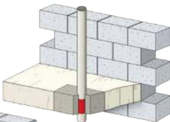
Floor Installation
