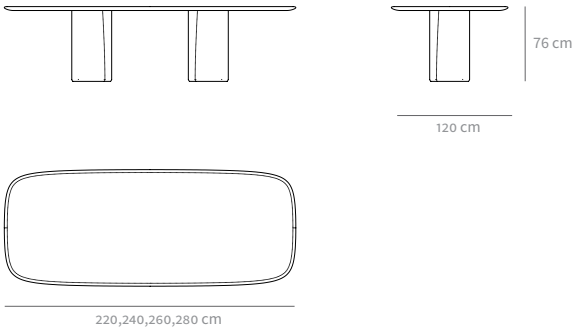
H 76 W 220, 240, 260, 280 D 120
