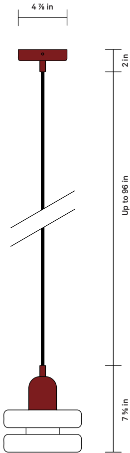
FRONT VIEW
