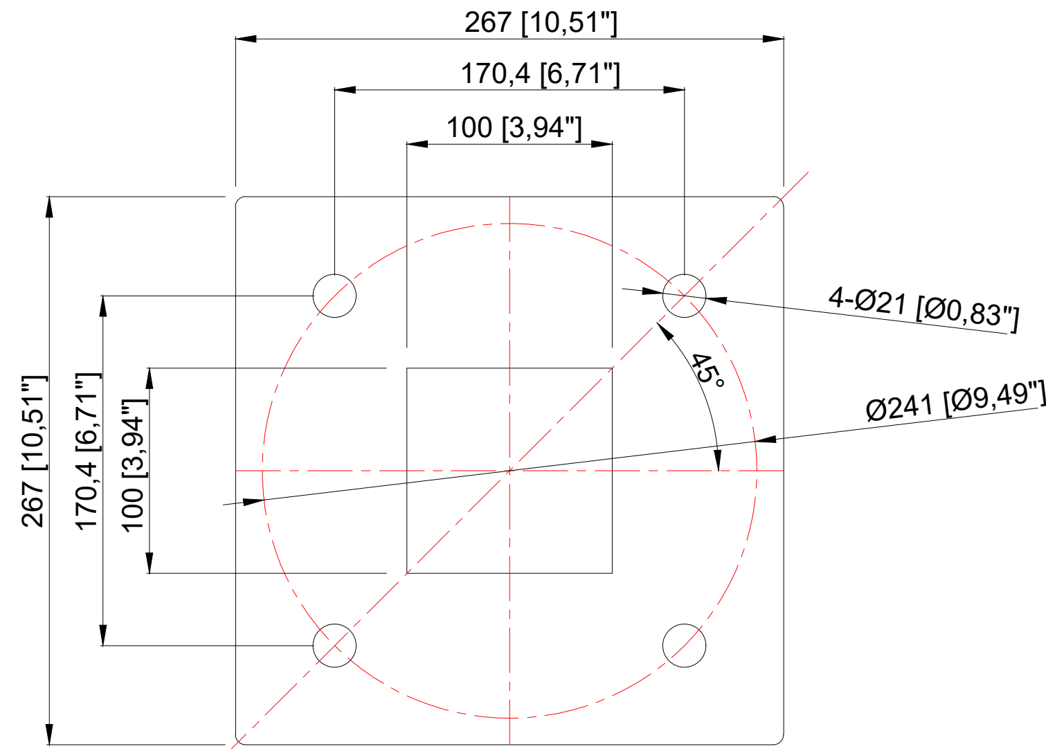
ANCHOR BOLT TEMPLATE
