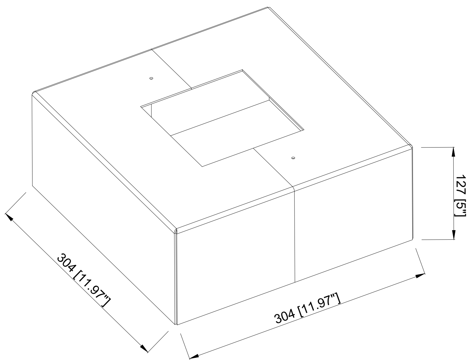
BASE COVER
