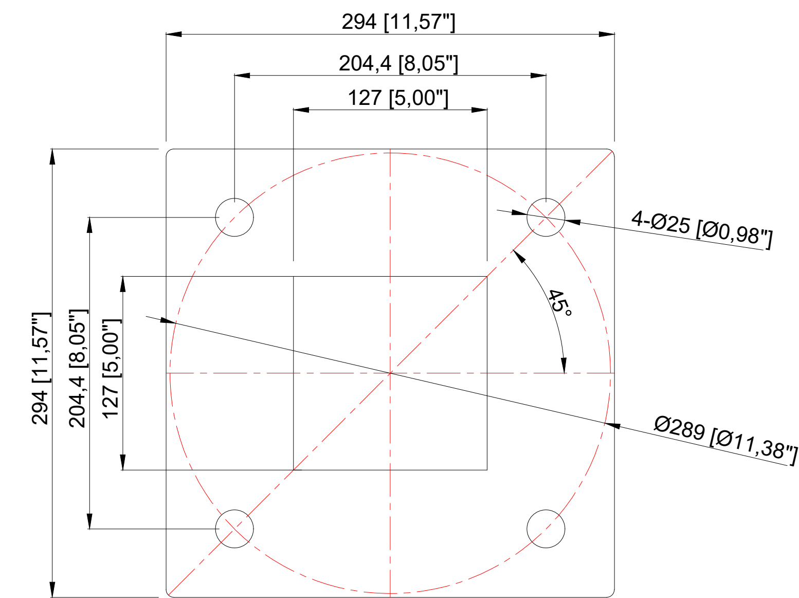
ANCHOR BOLT TEMPLATE
