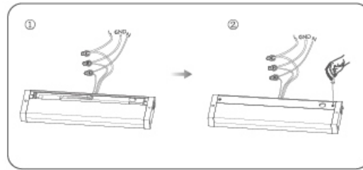
2. ① Connect -L/N/GND to the mains ② Screw the back cover
