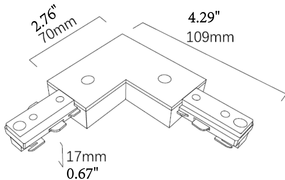
3 wire L connector
