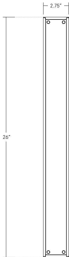
Elevation • Front
