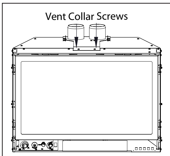
Figure 24: Vent Collar Plate Screw Location.
