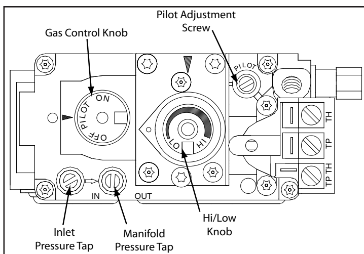
Figure 30: Valve Details.
