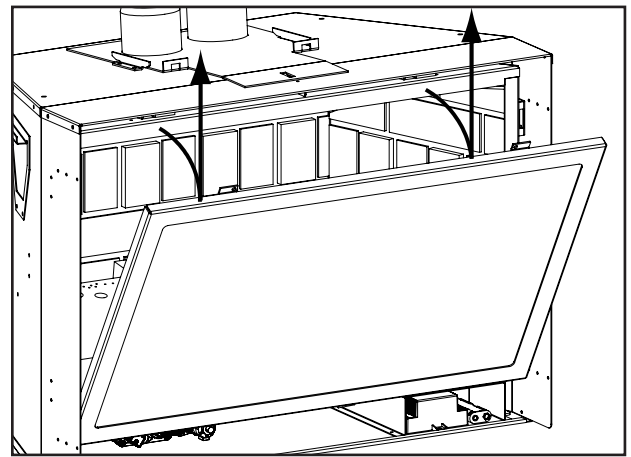
Figure 8: Door Removal.
