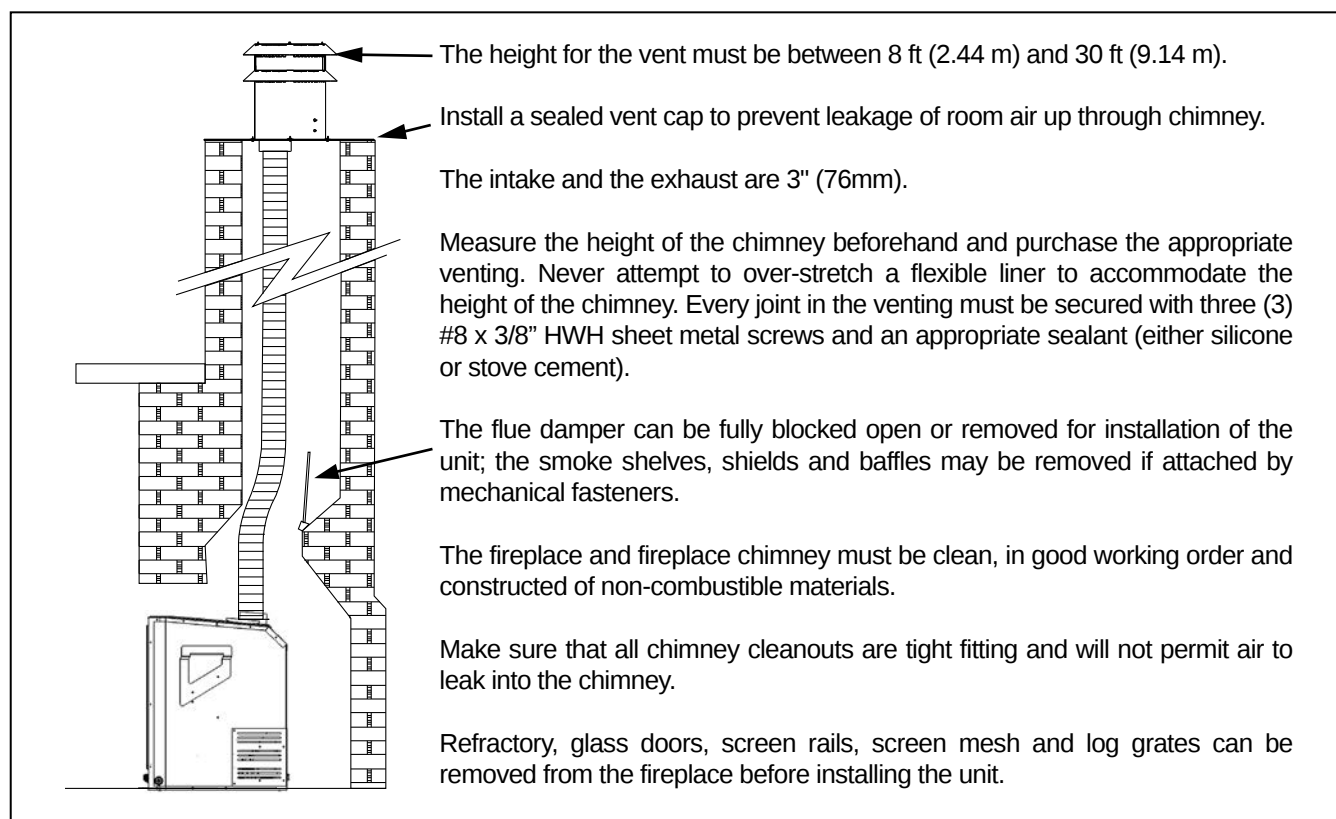
Figure 19: Installation of E30
