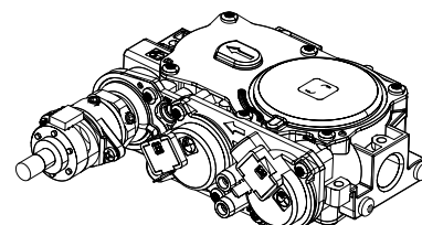
#50-2682 - SIT 885 VALVE W/ STEPPER MOTOR (NG)
