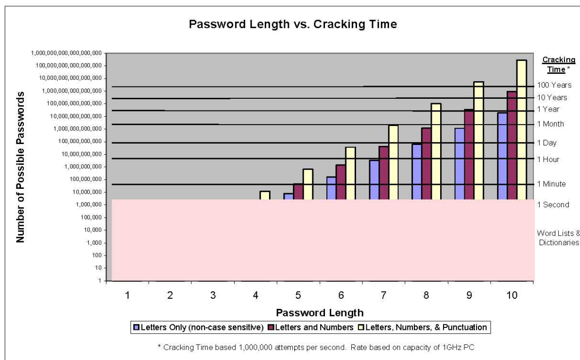
Figure 4 Password Length vs. Cracking Time
