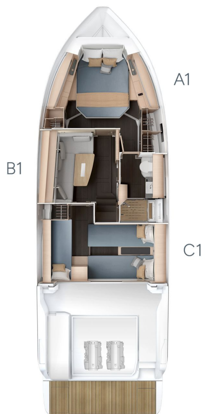
LOWER DECK
