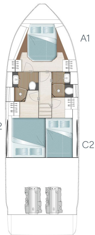
LOWER DECK
