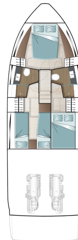
LOWER DECK
