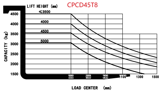
CAPACITY CHART
