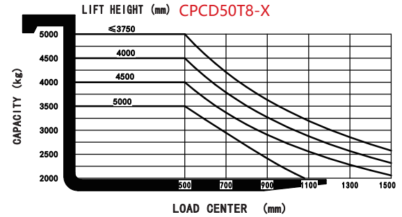
CAPACITY CHART
