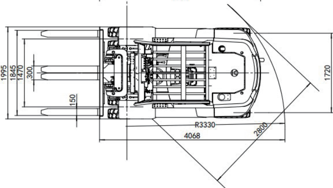
CPCD50T8
