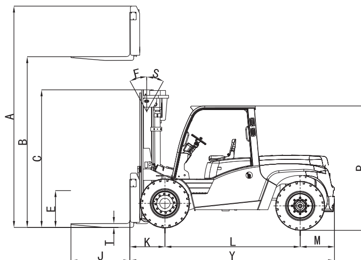
CPCD50T8
