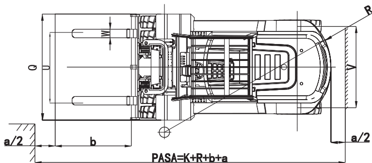
CPCD80-100T8
