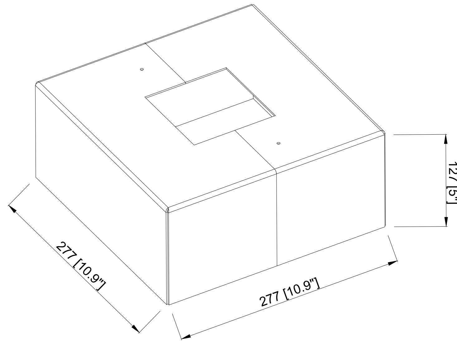
BASE COVER
