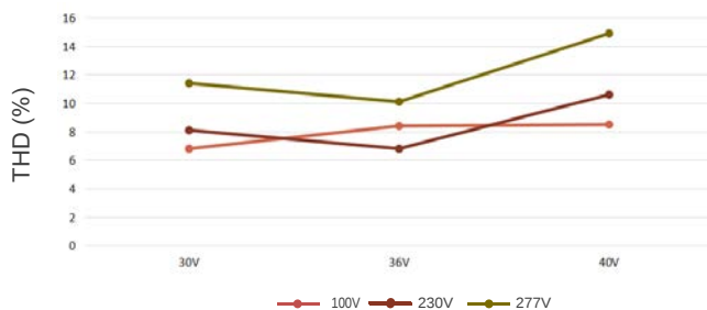
THD vs. Load
