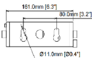
Yoke Mount
