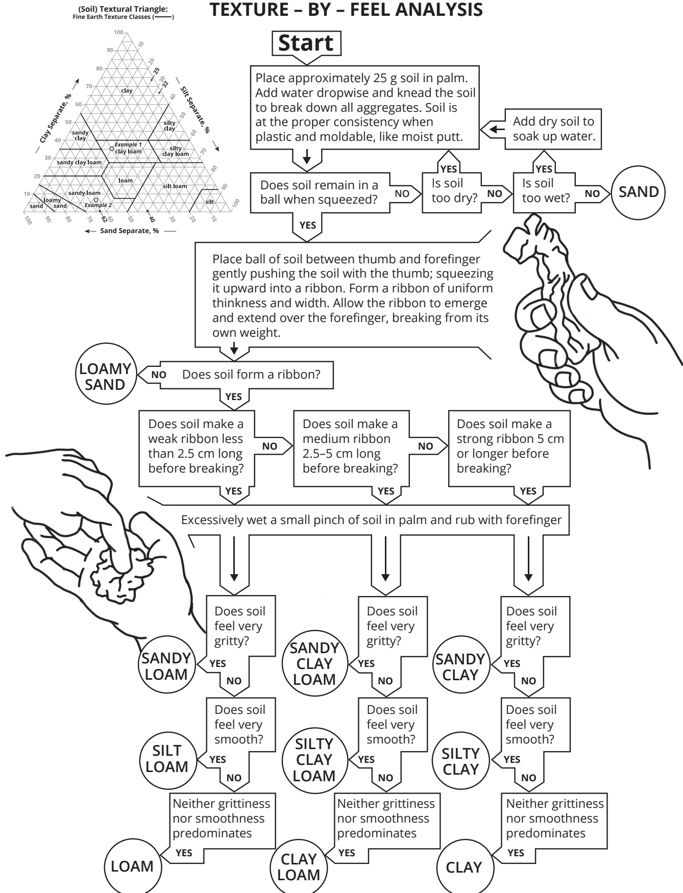
Figure 11. Soil Texture – The Field Feel Method
