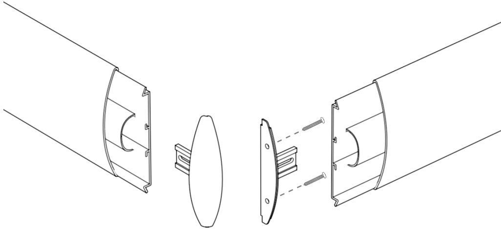
Corner Assembly
