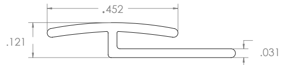
Joint Trim
