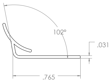
Inside Corner
