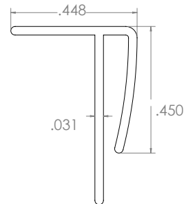
Outside Corner
