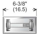
146 Front view
