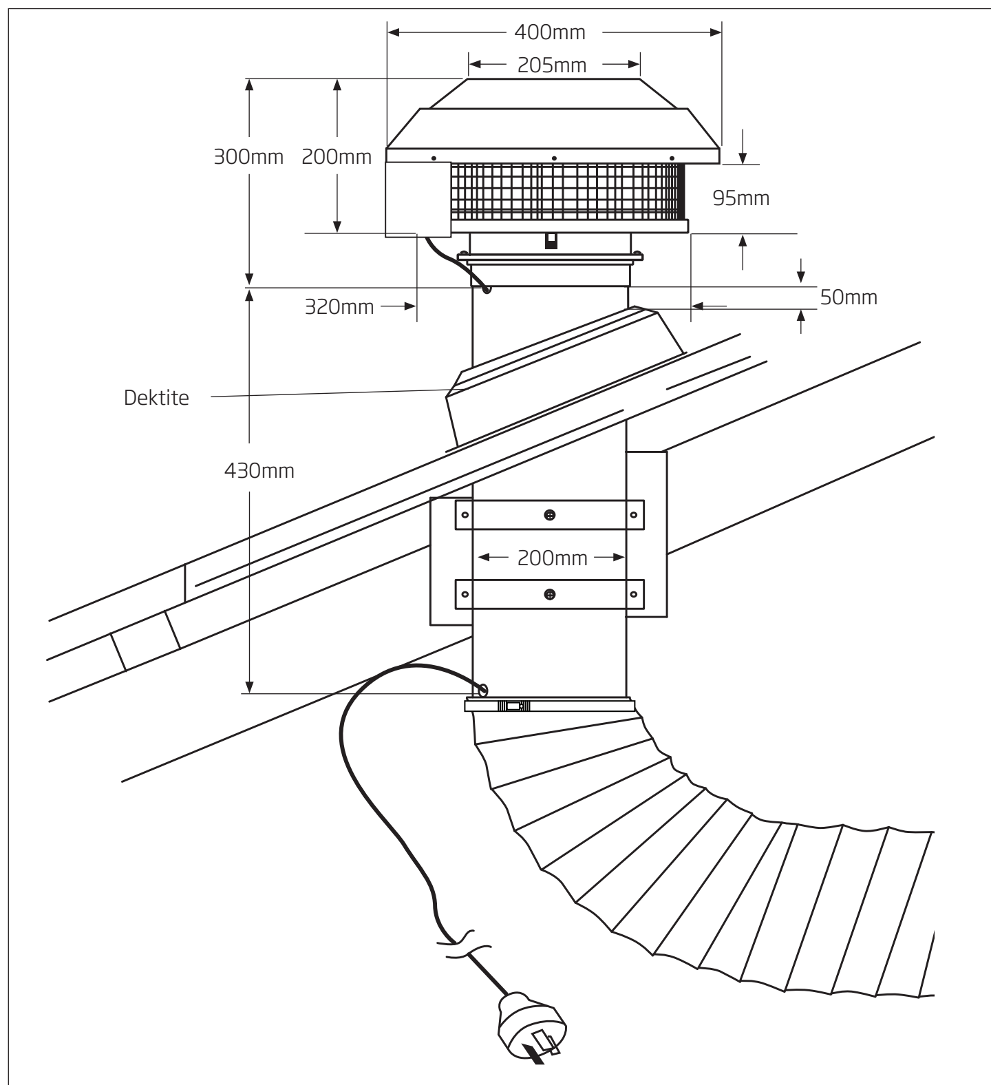
Figure 11: Dimensions for Isodrive 1650
