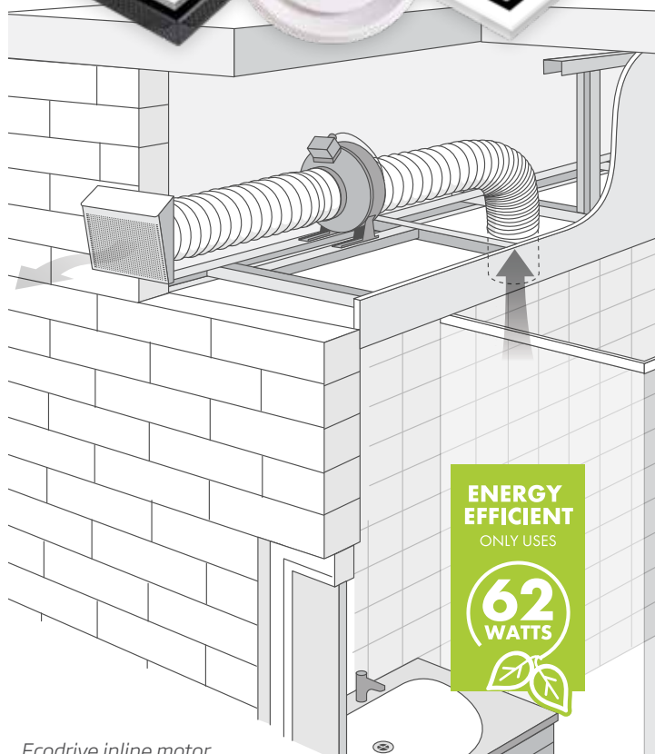
Ecodrive inline motor
