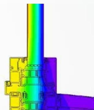
➤ F80 TEMPERATURE FIELD
