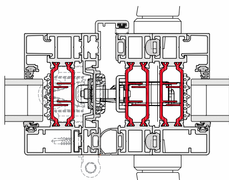
➤ F80 SLIM MEETING STILE - HALF ROLLER
