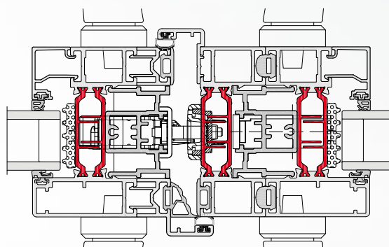
➤ F80 STANDARD FRENCH DOOR
