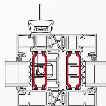
➤ F80 SLIM INTERLOCK
