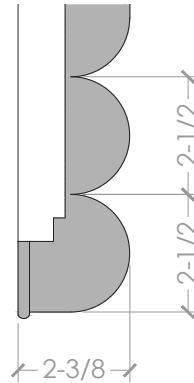
FRAME PROFILE
