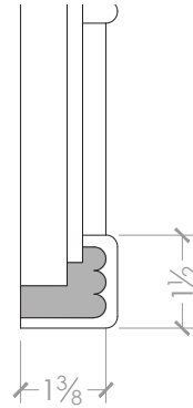
FRAME PROFILE
