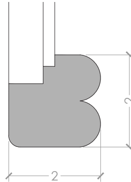
FRAME PROFILE
