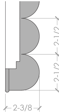
FRAME PROFILE
