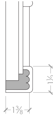
FRAME PROFILE
