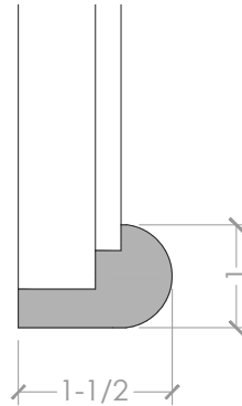
FRAME PROFILE
