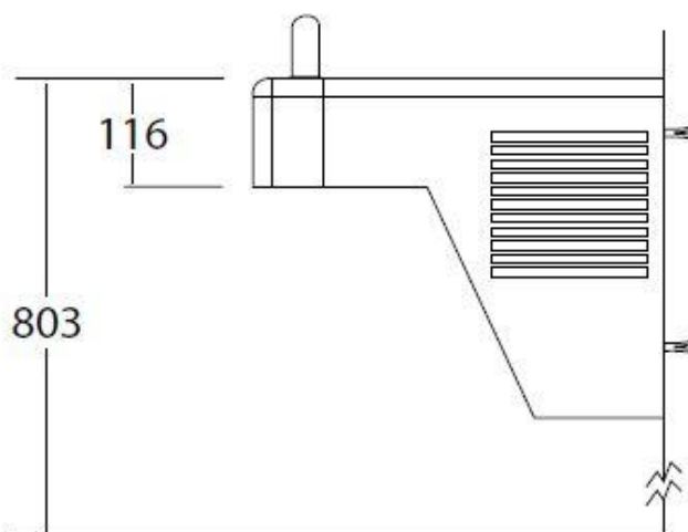
Side Plan
