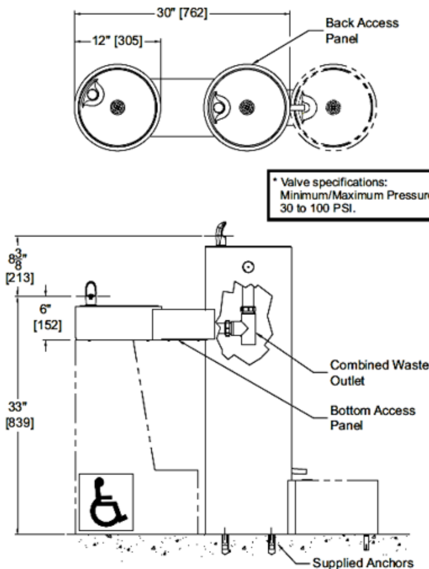
OPTIONAL -PF PET FOUNTAIN DETAIL
