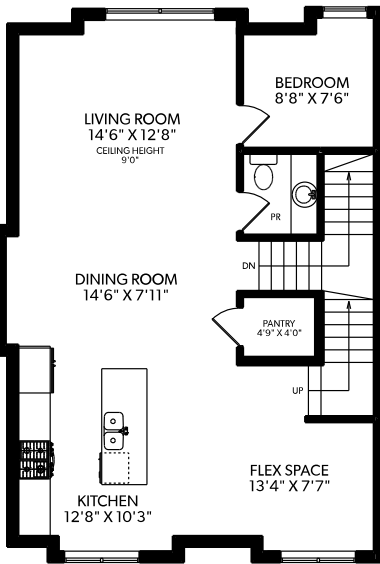
MAIN FLOOR
