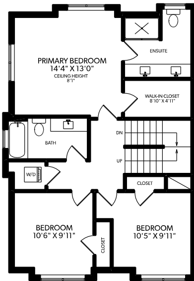
UPPER FLOOR
