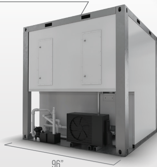
GALVANIZED-STEEL FRAME
