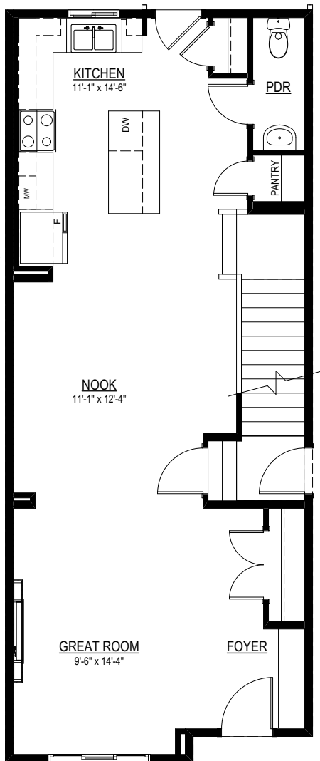
MAIN FLOOR
