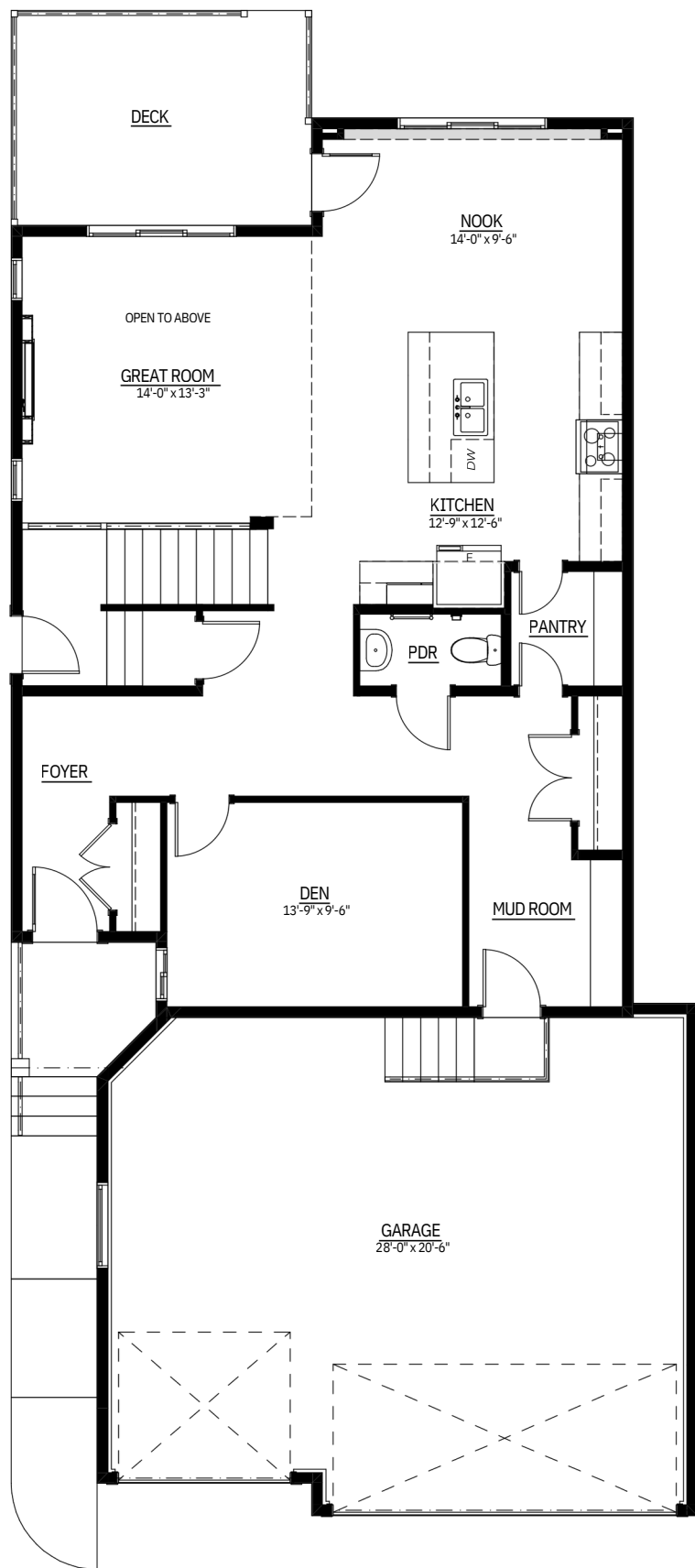
MAIN FLOOR
