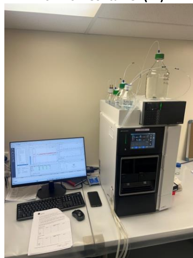
16139s - HPLC
