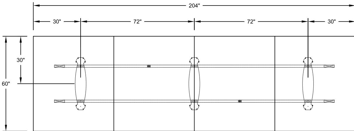
PLAN VIEW
