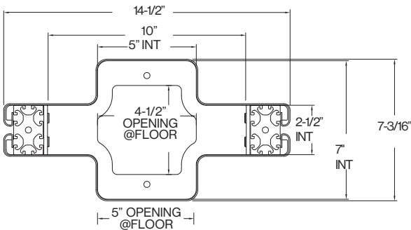
Plan View of Center Column base
