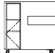
Combination of open shelves & hinged door with rolling screen
